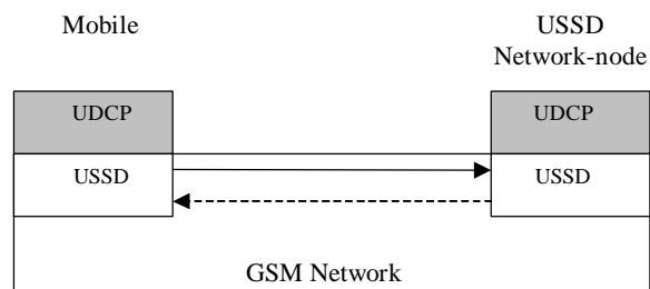
Figure 1 USSD and UDCP Architecture.
