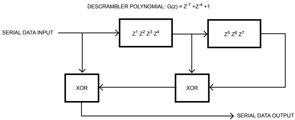
Figure 132 – Data descrambler
