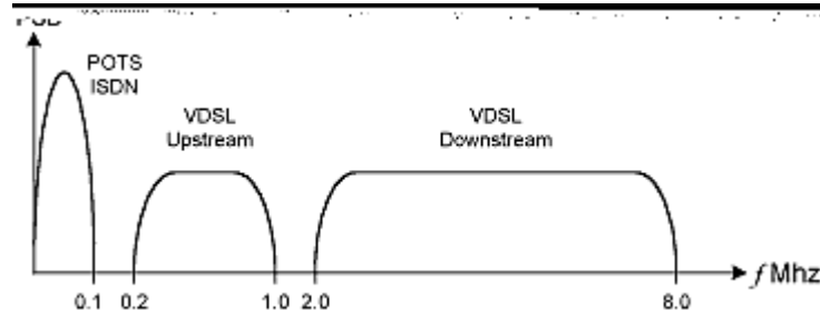
Figure 2. Example Single-Carrier VDSL Asymmetric Spectral Allocation
